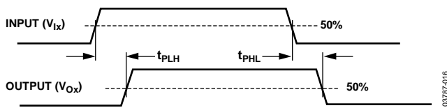
Figure 15. Propagation Delay Parameters
