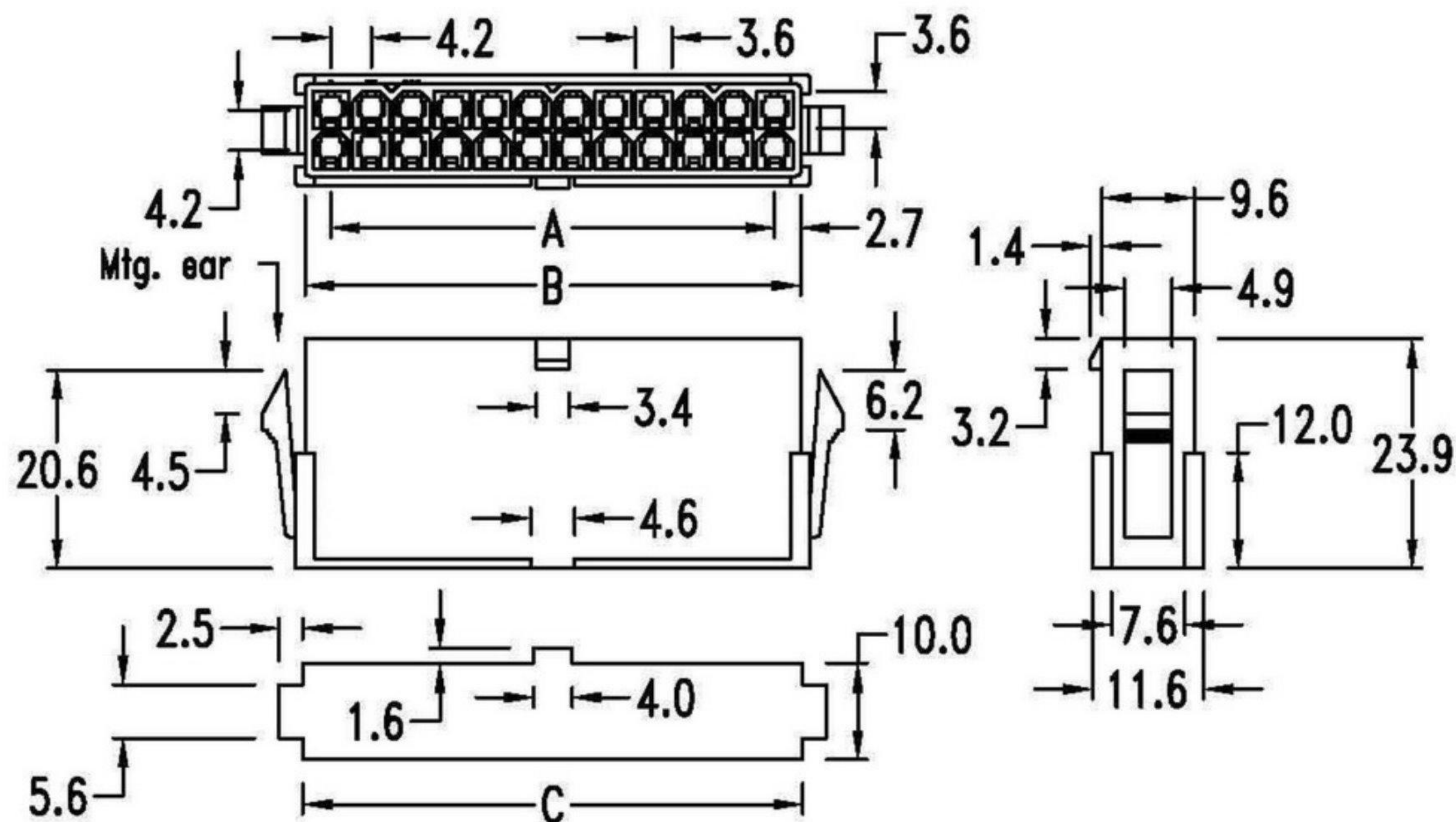
Dimensional Information ( mm )
