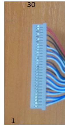
DF14-30S
