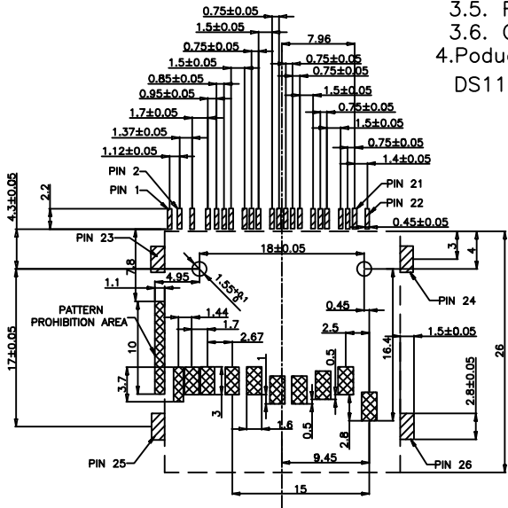
PCB LAYOUT
