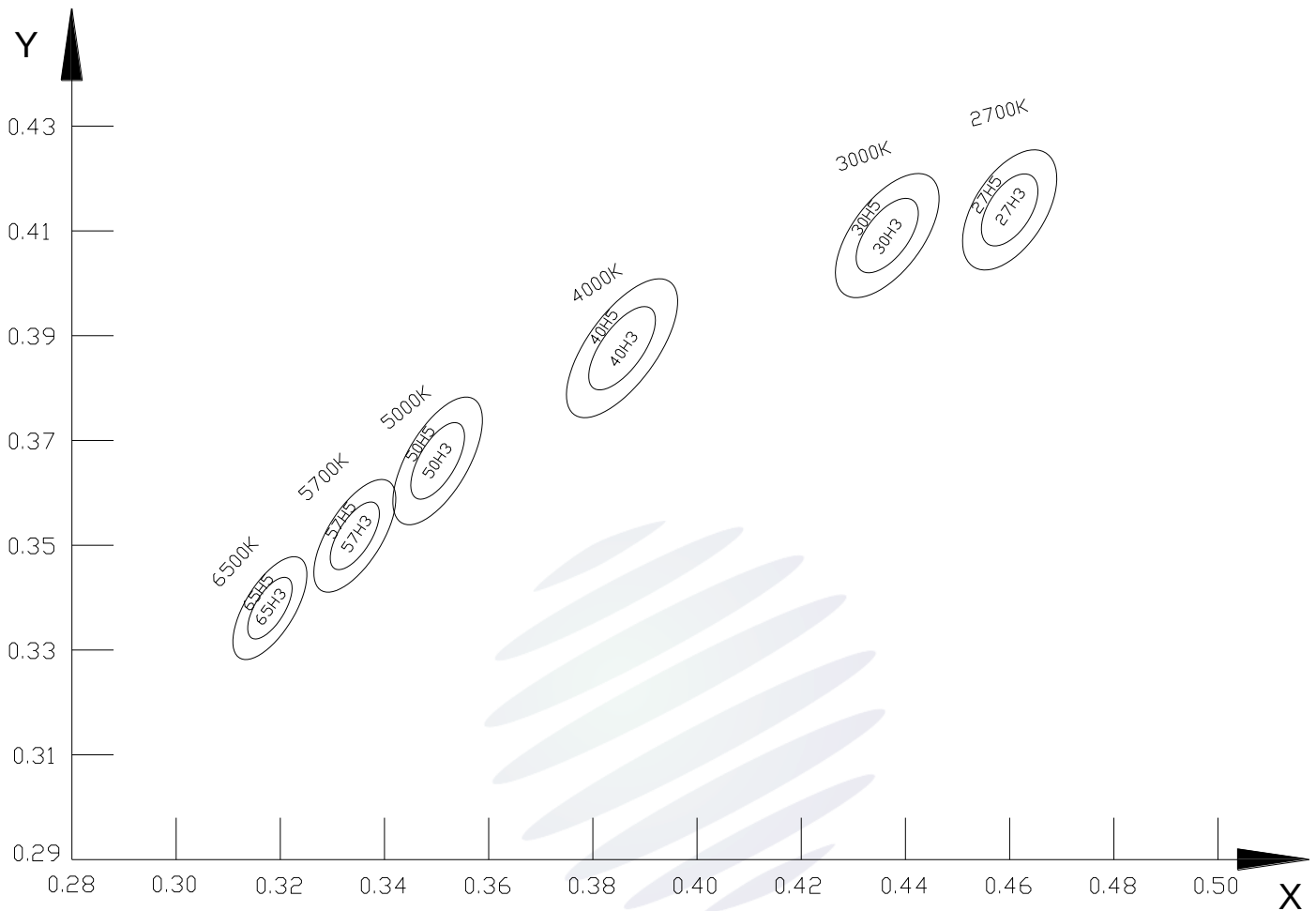
Fig 1-6 The C.I.E Chromaticity Diagram CIE色度图
