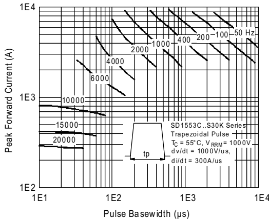
Fig. 37 - Frequency Characteristics
