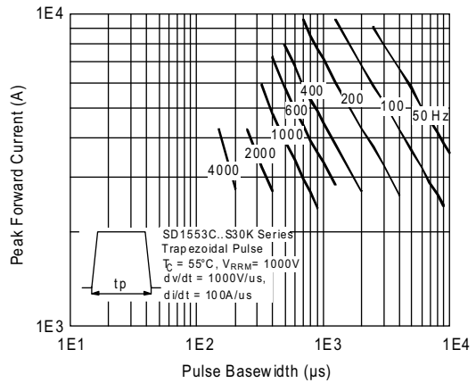
Fig. 39 - Frequency Characteristics
