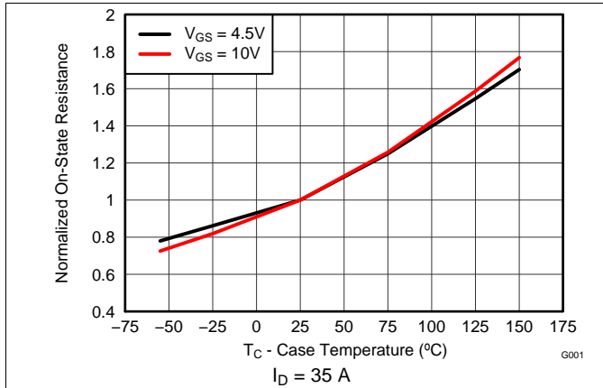
Figure 8. Normalized On-State Resistance vs Temperature
