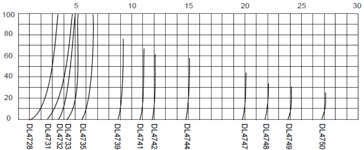
Breakdown Characteristics
