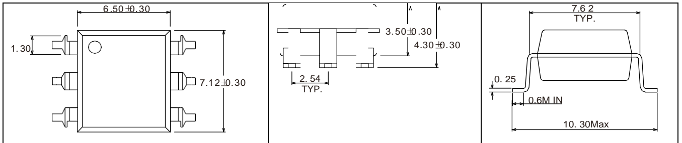
6-pin SOP
