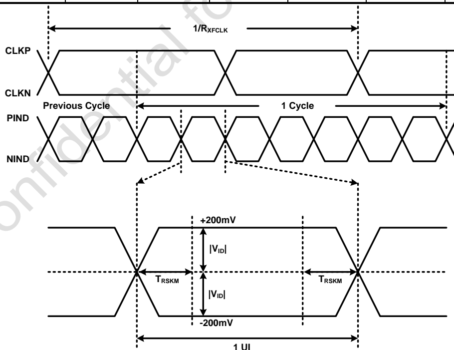
Fig. 5-3. LVDS AC characteristics diagram
