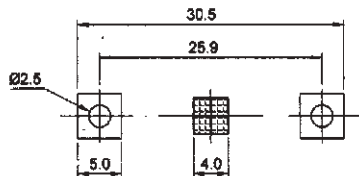
PCB Mounting layout
