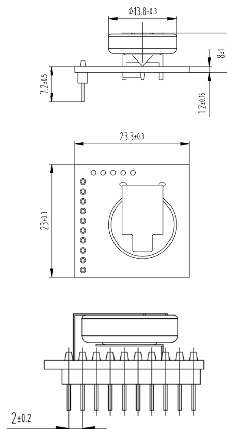
Fig1. Structure Unit: mm
