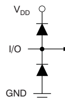
Equivalent Digital Input/Output Circuit
