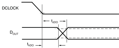
Voltage Waveforms for D_{OUT} Delay Times, t_{IDO}
