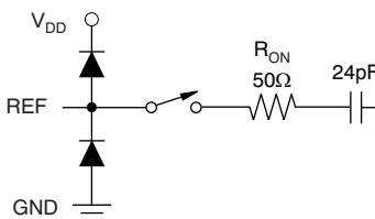
Equivalent Reference Input Circuit
