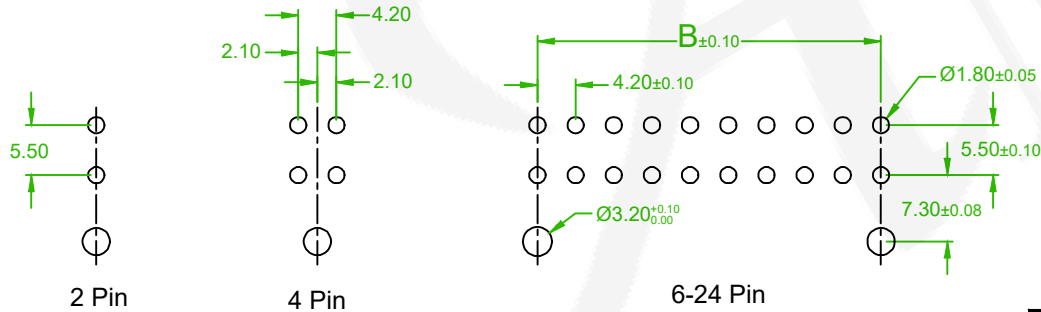
Recommended PCB Hole Layout PCB thickness: 1.78mm max.
