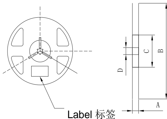
Fig.2-2 Reel Dimension 卷盘尺寸
