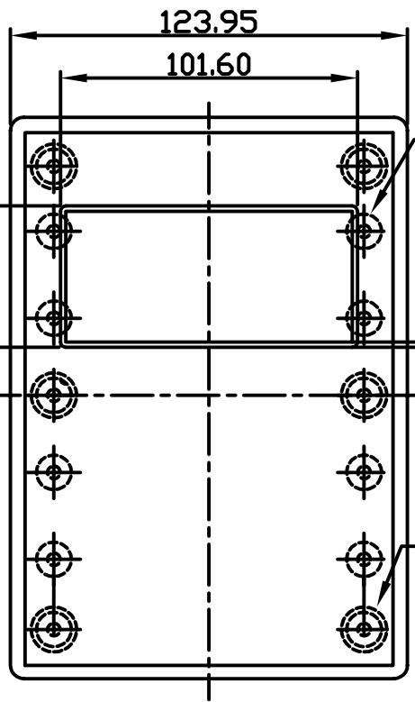
BOTTOM VIEW
