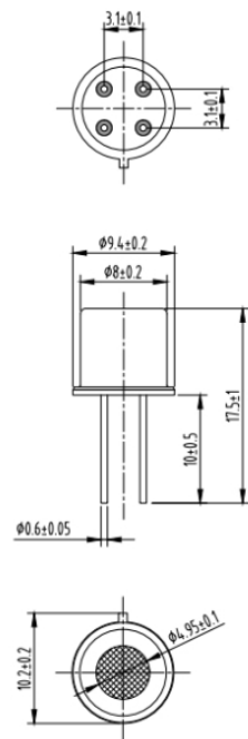
Fig1.Sensor Structure
