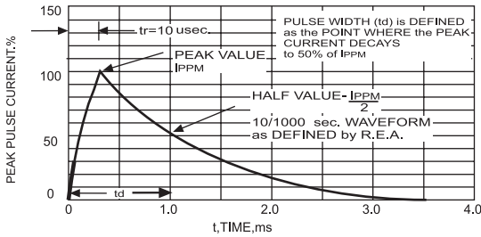
FIG.3- PULSE WAVEFORM
