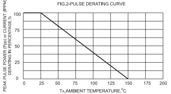
FIG.2-PULSE DERATING CURVE
